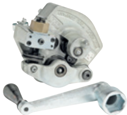
Manual Operation with Ratchet Handle
