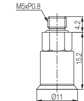
With M5M fitting
