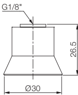
With 1/8F fitting
