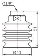
With 18FB fitting
