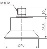
With M10M fitting
