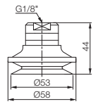
With 18F fitting
