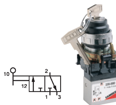
3/2 3 Key Switch
