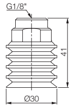
With 18FB fitting
