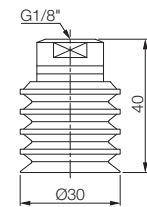
With 18F fitting
