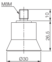
With M8M fitting
