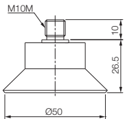
With M10M fitting
