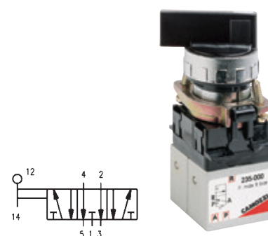
5/3 3 Position Selector Switch
