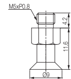
With M5M fitting
