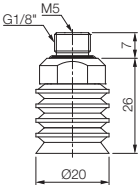
With M518MB fitting
