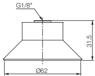
With 18F fitting
