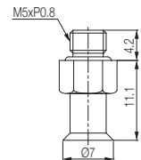
With M5M fitting
