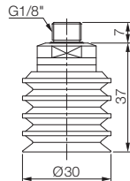
With 18M fitting
