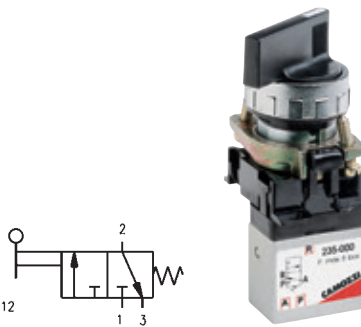
3/2 2 Position Selector Switch
