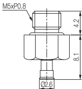
With M5M fitting
