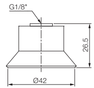
With 18F fitting
