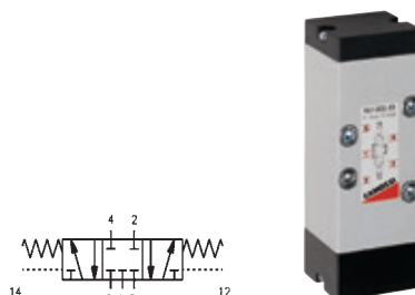
5/3 Pneumatic Closed Centres (961, 962 & 963)
