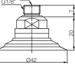
With M518MFX fitting
