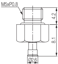
With M5M fitting
