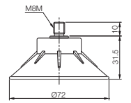
With M8M fitting
