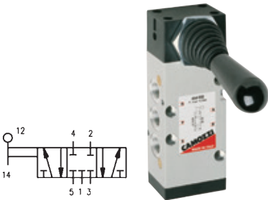
G1/4", 5/3 CC Lever Valve Bistable
