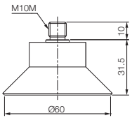
With M10M fitting
