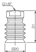
With 18F fitting
