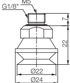
With M518MFB fitting
