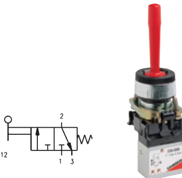
3/2 Joystick Valve
