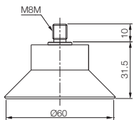
With M8M fitting
