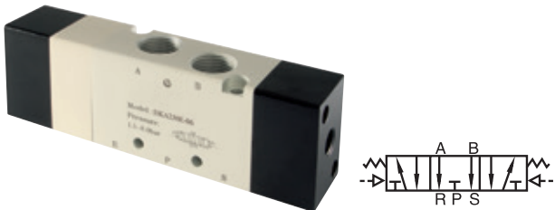
Pilot/Pilot, Supply Sealed Mid Position, BSPP
