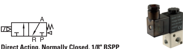
Direct Acting, Normally Closed, 1/8" BSPP
