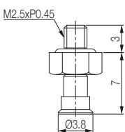
With M2.5M fitting
