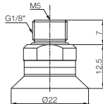
With M518MFO fitting
