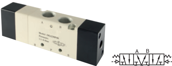
Pilot/Pilot, Centre Open Pressurised, BSPP
