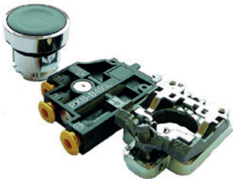
Push Button & Valve Spring Return 4mm Push-in
