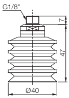
With 18M fitting
