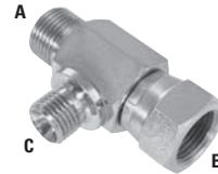
BSPP Male x BSPP Swivel Female x BSPP Male Branch Tee Reducing on Branch 60° Cone
