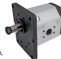
1:8 Taper Shaft, 4 Bolt European Flange, SAE Ports, Clockwise Rotation
