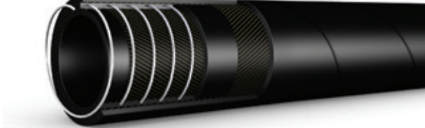
100R4 - 3/4" OIL SUCTION & DE
